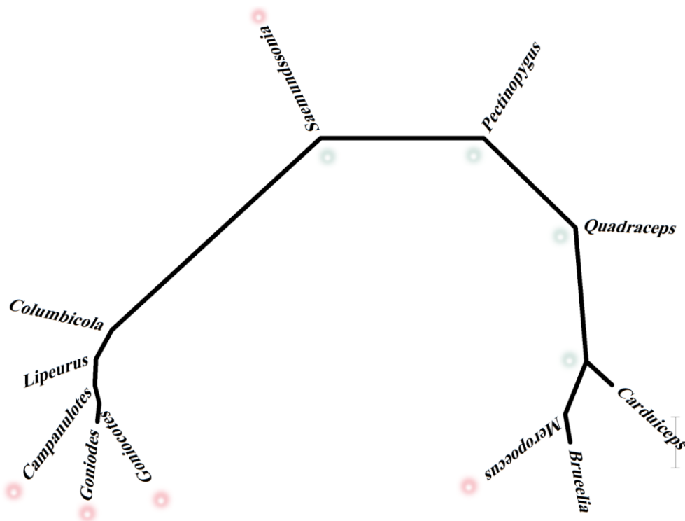
Figure 3. Unrooted tree based on Neighbor-Joining analysis of COI gene and elongation factor-1 alpha gene alignments for all recorded Saudi Arabia genera of Ischnocera (Red flash indicates head chewing lice; Blue flash indicates aquatic chewing lice).
