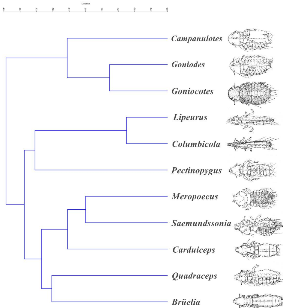
Figure 1. Phylogenetic tree based on Neighbor-Joining classification using Euclidean distance of morphological and ecological Data matrix for all recorded genera of Ischnocera.
