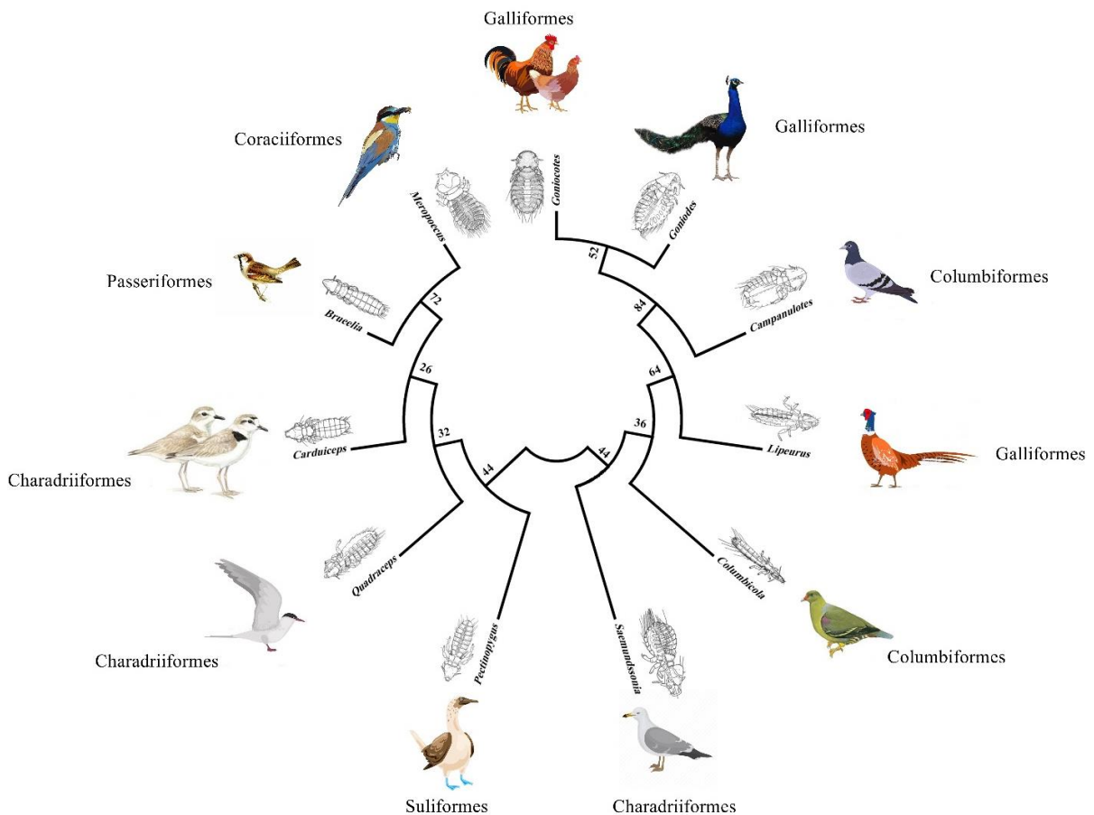
Figure 2. Phylogeny tree based on Neighbor-Joining analysis of COI gene and (EF-1) gene alignments for all recorded genera of Ischnocera.
