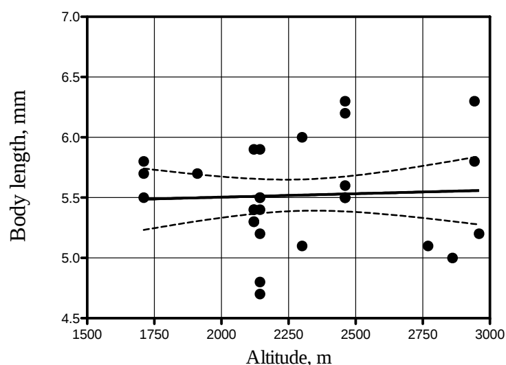
Figure 5. Linear regression of body length distribution of Chrysella tatiana Semenov, 1967 as a function of altitude. The continuous line shows the linear fit of data and the broken lines the confidence interval of 95%.
