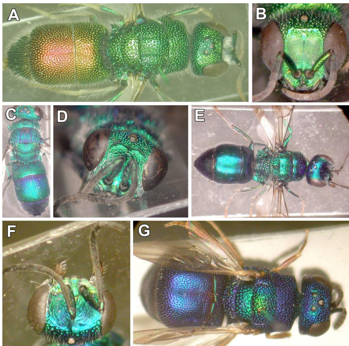
Figure 3. Chrysis sacrata Buysson, 1898: A. body, dorsal view; B. head, frontal view; Chrysis quadrispina Buysson, 1887; C. body, dorsal view; D. head, frontal view; Elampus kashmirensis Nurse, 1902; E. body, dorsal view; F. head, frontal view; G. Holopyga chrysonota appliata Linsenmaier, 1959. Male from Kerman, Baft-Anjerk, 21.05.2016, 2148m, 29°9'35"N-56°46'00"E, M. Purrezaali.
