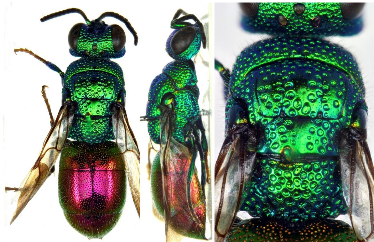
Figure 2. Female of Chrysellampus tatianae Semenov, 1967 from Kerman province;: Qal-eh-Askar, 1911m, 14.05.2015, 29°44'39.2"N56°45.25'3"E, swept on Medicago sativa , leg. S. Safahani. From left: dorsal view, lateral view and magnification of mesonotum dorsum.
