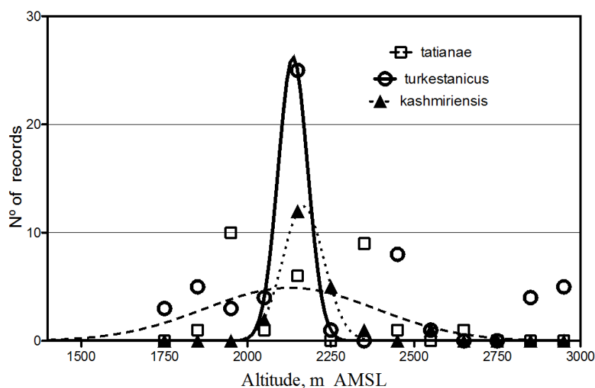
Figure 4. Altitude distribution of three Chrysidae species from Kerman Mountains: Chrysella tatiana Semenov, 1967 (broken line), Pseudomalus turkestanicus Mocsáry, 1889 (continuous line), and Elampus kashmirensis Nurse, 1902 (pointed line).
