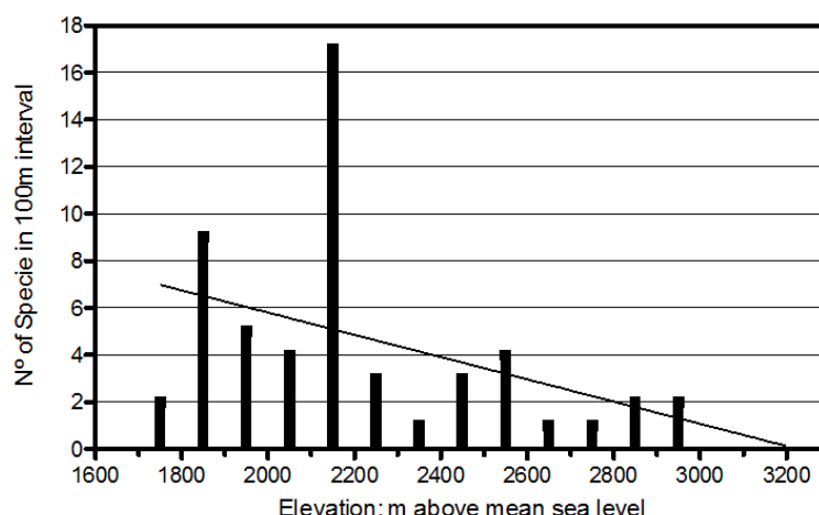
Figure 6. Linear regression of Chrysididae altitudinal distribution in Kerman Mountains (Iran).
